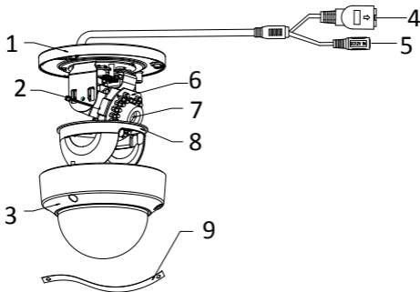
Figure 1-1 Camera Overview
