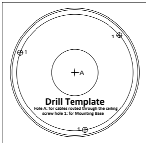
Figure 2-1 Drill Template
