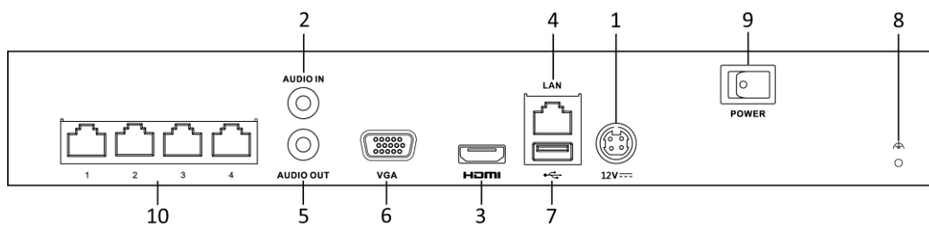
Figure 1-4 DS-7600NI-Q1/4P Series
