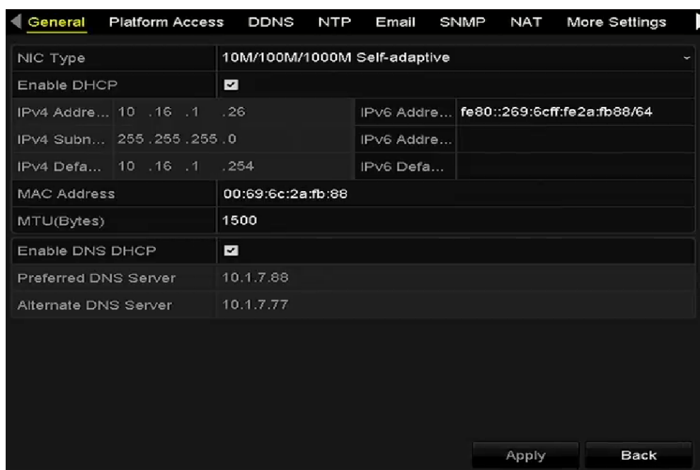
Figure 3-9 Network Settings
