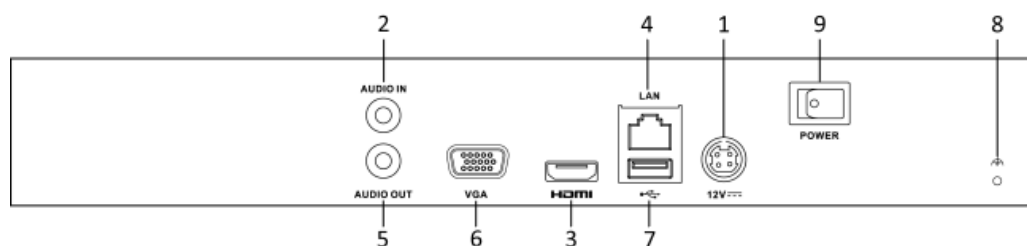
Figure 1-3 DS-7600NI-Q1 and DS-7600NI-Q2 Series
