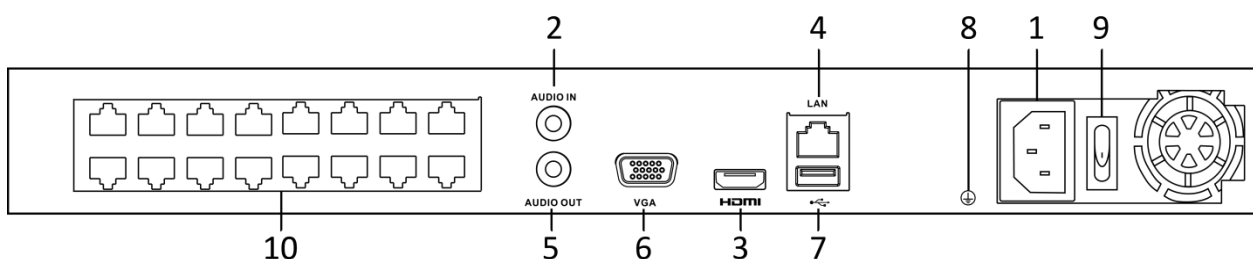
Figure 1-5 DS-7600NI-Q2/16P Series
