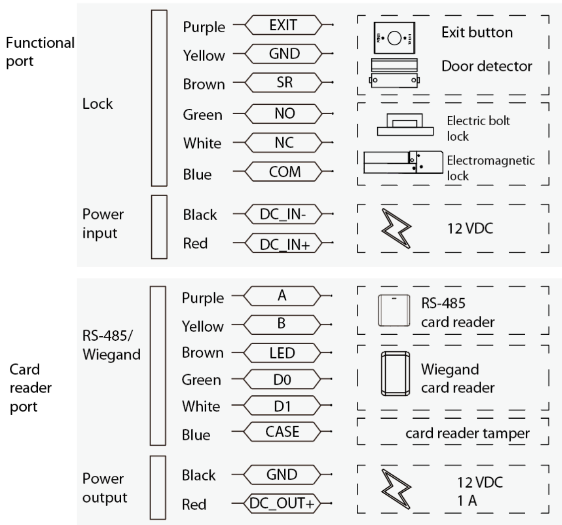
Figure 2-4 Cables
