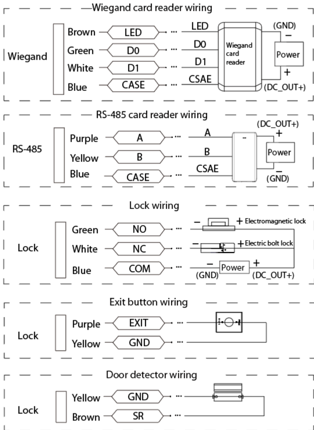
Figure 2-5 Wiring
